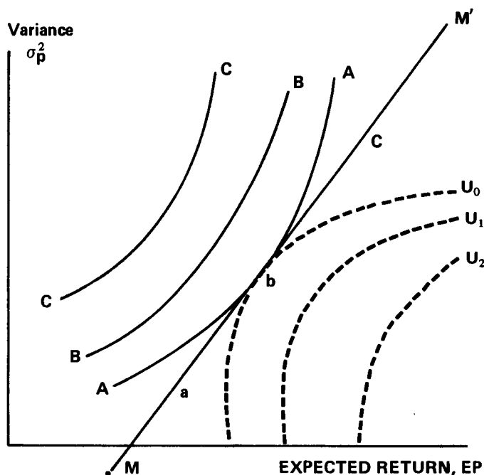
FIGURE 1 EFFICIENT FRONTIERS IN PORTFOLIO SELECTION
